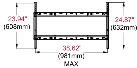
ADAPTOR BRACKET
