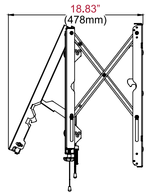
SIDE VIEW EXTENDED
