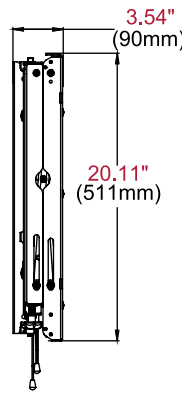
SIDE VIEW COLLAPSED
