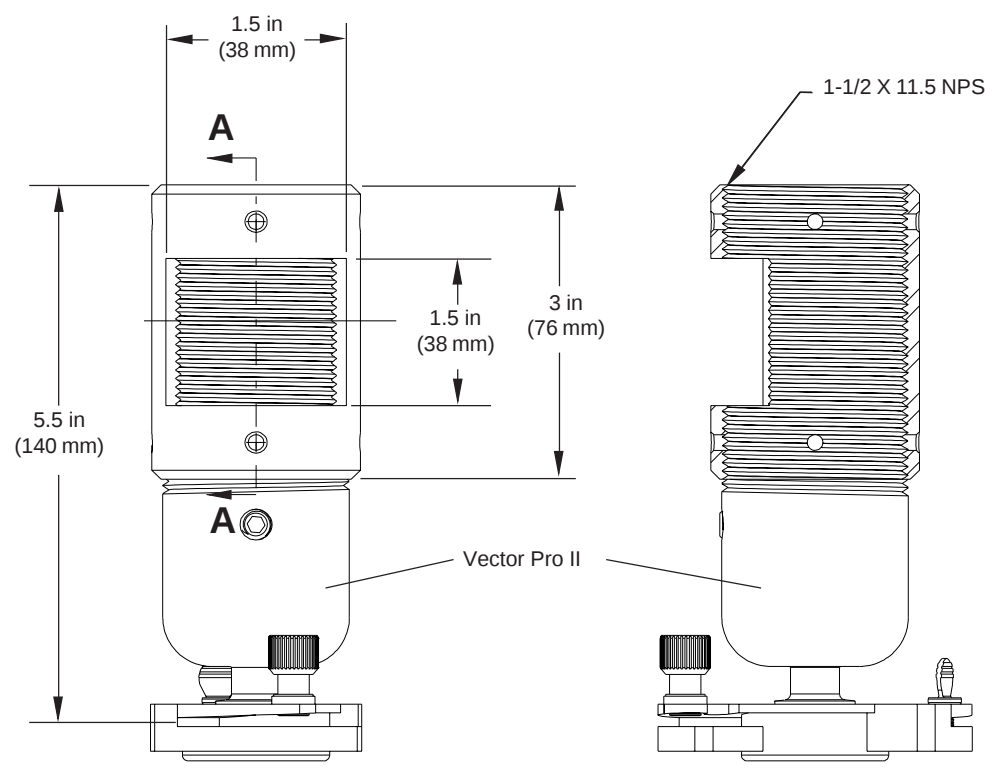
FRONT VIEW SECTION A-A WITH CORD MANAGEMENT CONNECTOR
